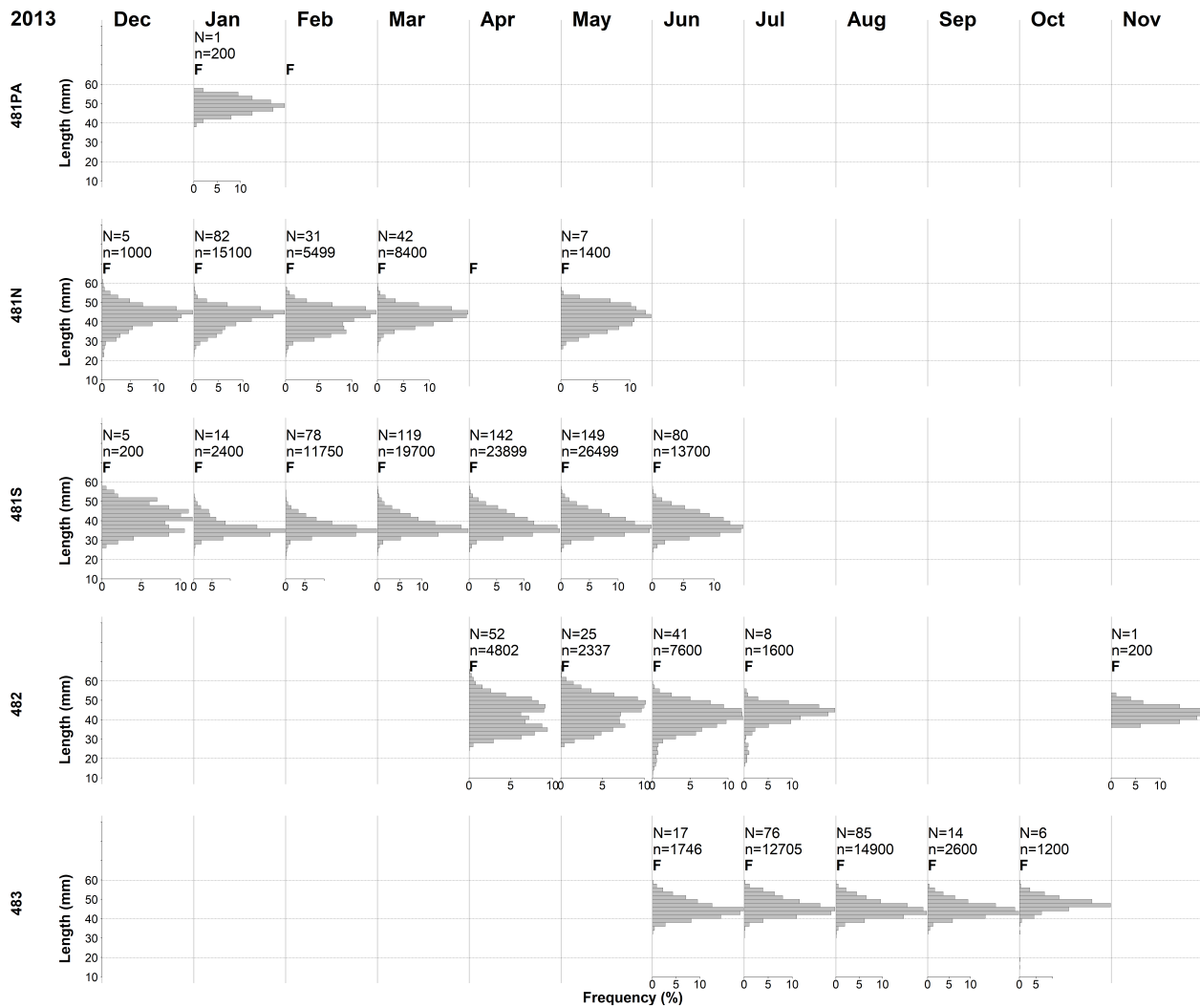
Figure A1. Monthly length frequency distributions for krill in Subareas 48.1 (including PA, N and S), 48.2 and 48.3 in 2013. The number of hauls from which krill were measured (N) and the number of individuals measured (n) in each month are provided; the months in which fishing occurred in a subarea are indicated by the letter F.
