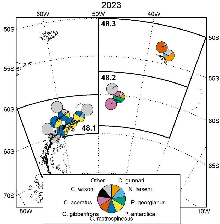
Figure 9. Distribution of estimated by-catch weight proportions for dominant fish species from the SISO data for 2023 (inspected hauls only). Records were pooled in 150 km grid cells prior to computing proportions. Coastlines and ice shelves: UK Polar Data Centre/BAS and Natural Earth. Projection: EPSG 6932 (rotated).
