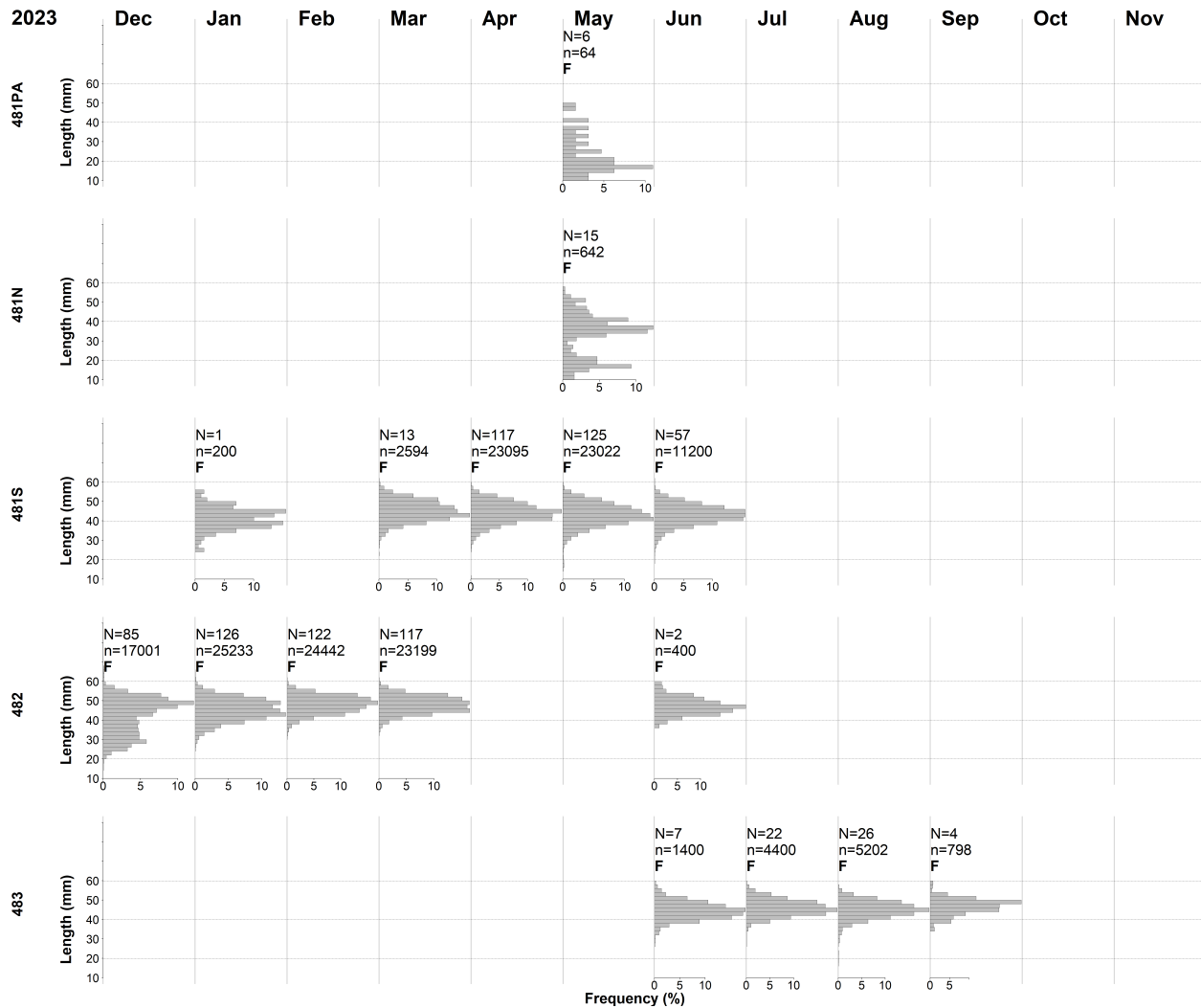
Figure 12. Monthly length frequency distributions for krill in Subareas 48.1 (including PA, N and S), 48.2 and 48.3 in 2023. The number of hauls from which krill were measured (N) and the number of individuals measured (n) in each month are provided; the months in which fishing occurred in a Subarea are indicated by the letter F.
