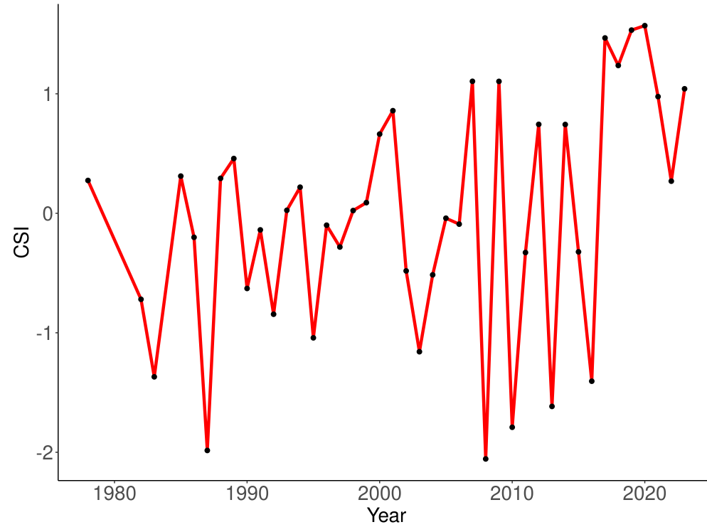
Figure 13. Combined Standardised Index time series from CEMP parameters collected at Admiralty Bay, Cape Shireff, Esperanza Station, Goudier Island, Stranger Point Station for Adelie, gentoo and chinstrap penguins, and fur seals in Subarea 48.1.
