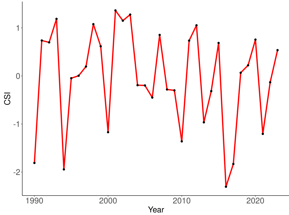
Figure 14. Combined Standardised Index time series from CEMP parameters collected at Laurie Island and Signy Island for Adelie and chinstrap penguins in Subarea 48.2.
