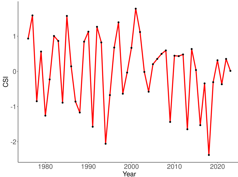
Figure 15. Combined Standardised Index time series from CEMP parameters collected at Bird Island and Maiviken for macaroni and gentoo penguins, southern black browed albatross, and fur seals in Subarea 48.3.
