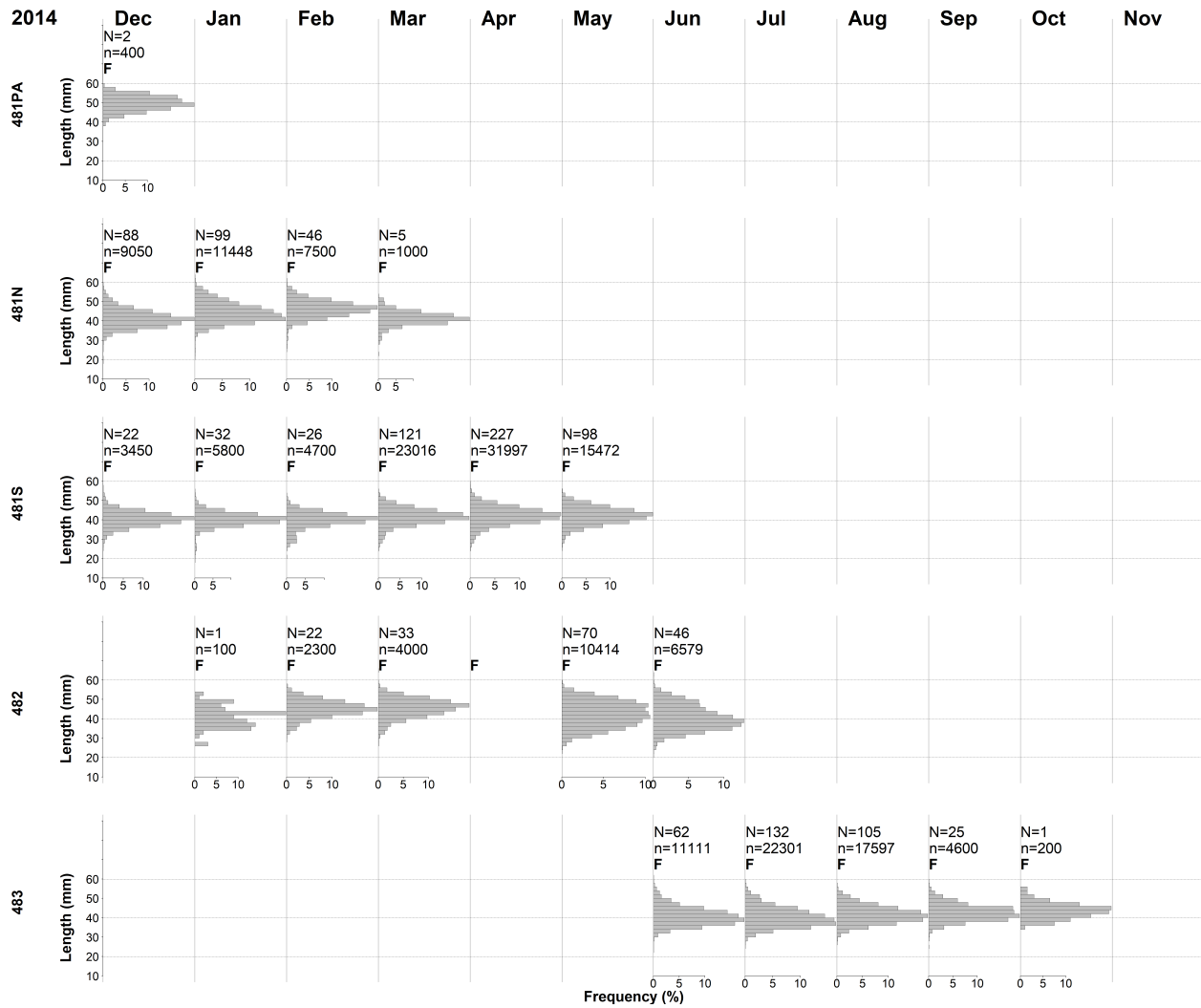
Figure A2. Monthly length frequency distributions for krill in Subareas 48.1 (including PA, N and S), 48.2 and 48.3 in 2014. The number of hauls from which krill were measured (N) and the number of individuals measured (n) in each month are provided; the months in which fishing occurred in a subarea are indicated by the letter F.
