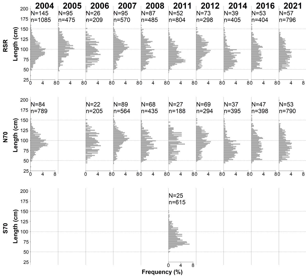
Figure 3. Annual length frequency distributions of D. eleginoides caught in this fishery (RSR; Subarea 88.1 and SSRUs 882A-B) (top panel) and two other areas of the fishery. The number of hauls from which fish were measured (N) and the number of fish measured (n) in each year are indicated. Note: length frequency distributions are only shown where more than 150 fish were measured in a given season/area.
