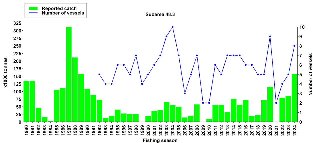
Catch and effort history in Subarea 48.3. The number of active vessels before 1992 is uncertain.
