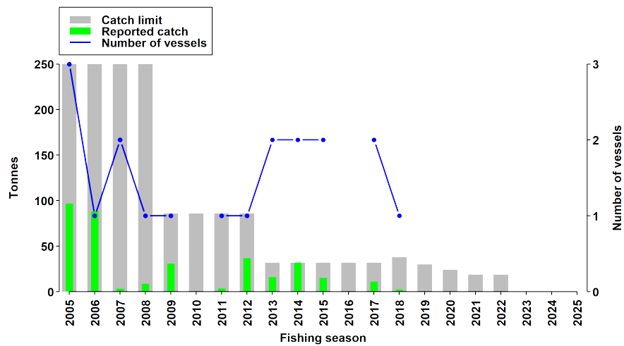
Catch and effort history in Division 58.4.3a.
