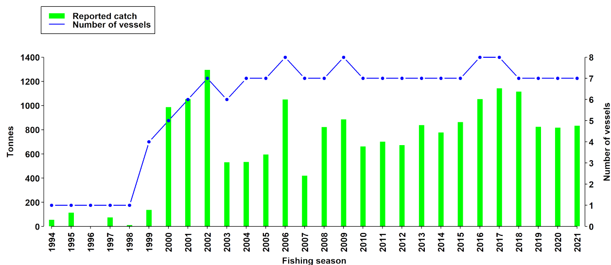
Catch and effort history at Crozet Island French EEZ (Subarea 58.6)
