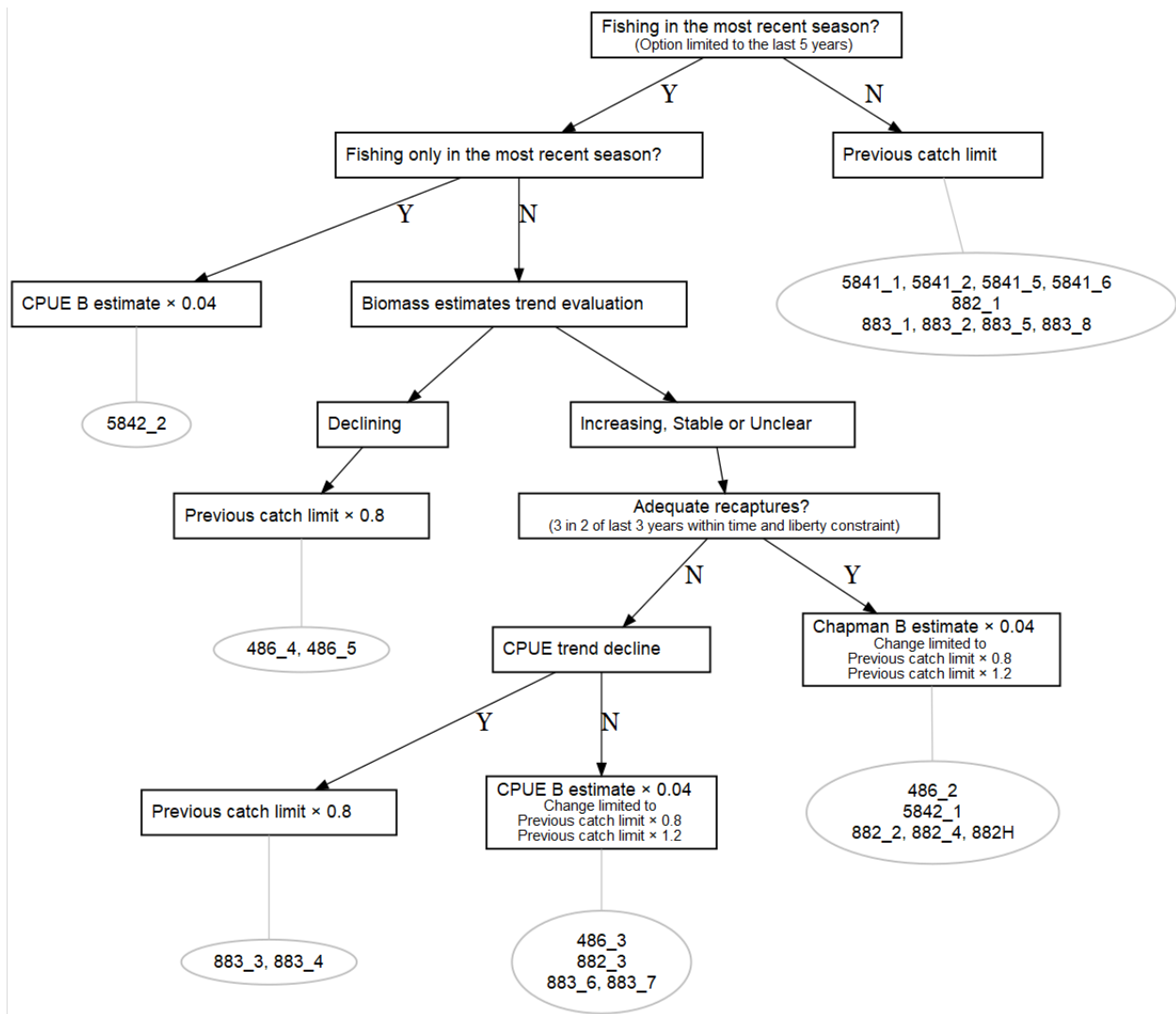
Figure 5: The decision tree of the trend analysis, showing where each Research Block (grey ovals) requiring catch advice belongs this year.
